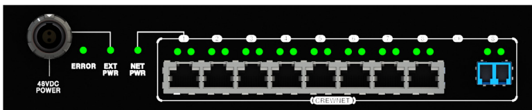
CHB-8C-02: Copper Hub Rear View
