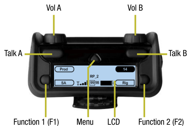
Radio Pack (CRP-22) Top View
