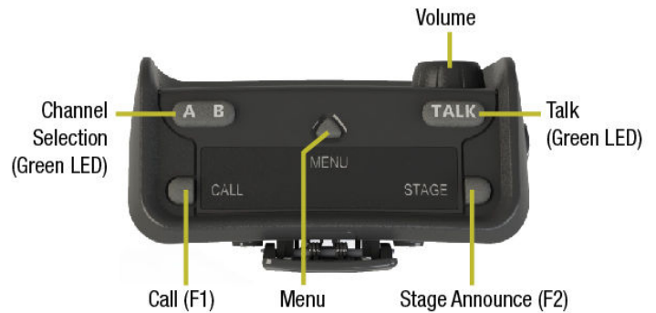
Radio Pack (CRP-12) Top View
