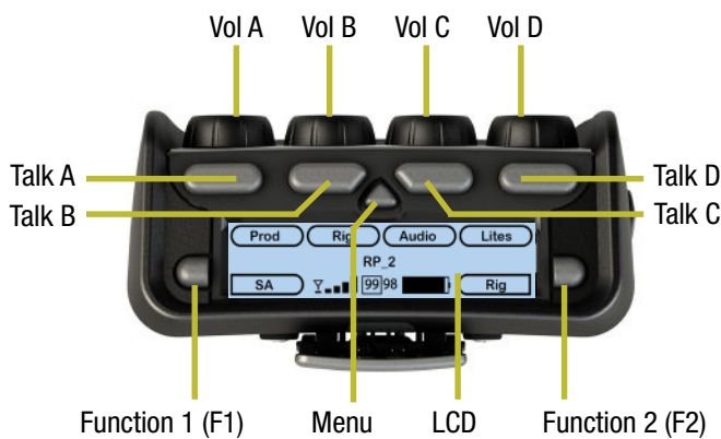
Radio Pack (CRP-44) Top View
